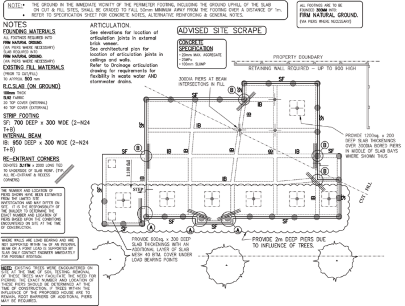
Fig 3 - example of footing plan
