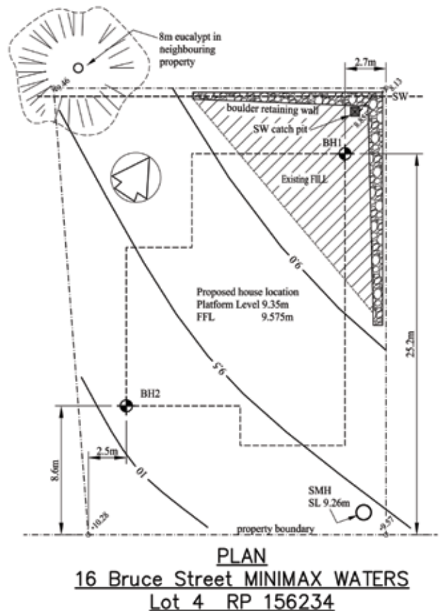
Fig. 1 - Example of site identification plan
